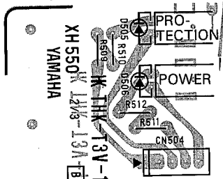
Components side
